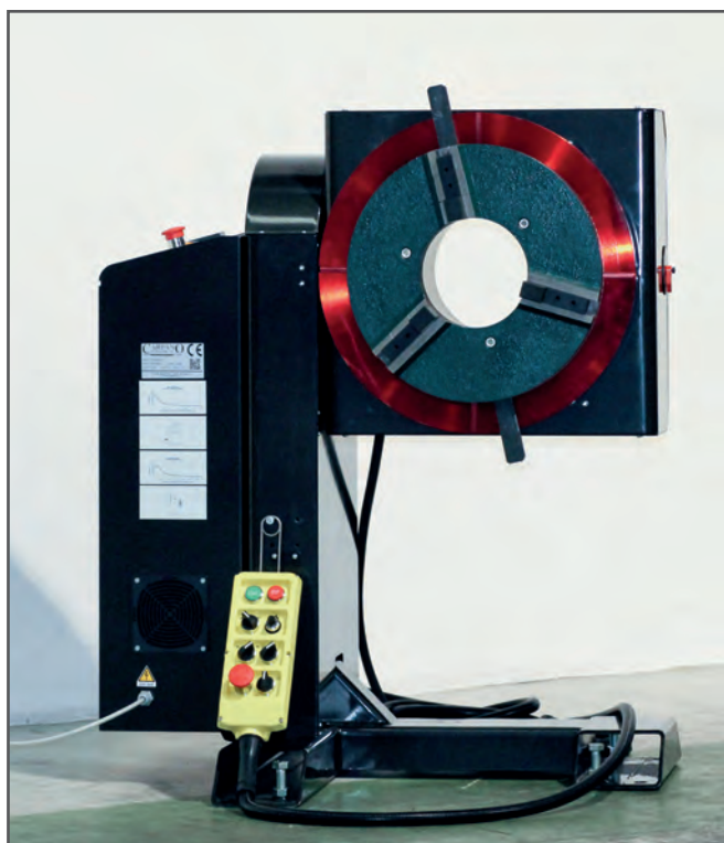
Front view, with Grip400 chuck
